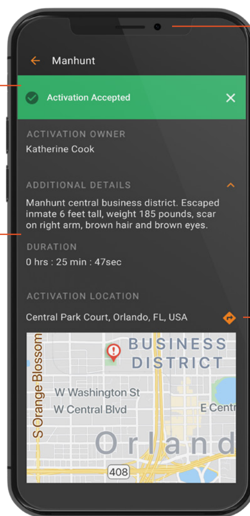
ACTIVATION SCREEN
